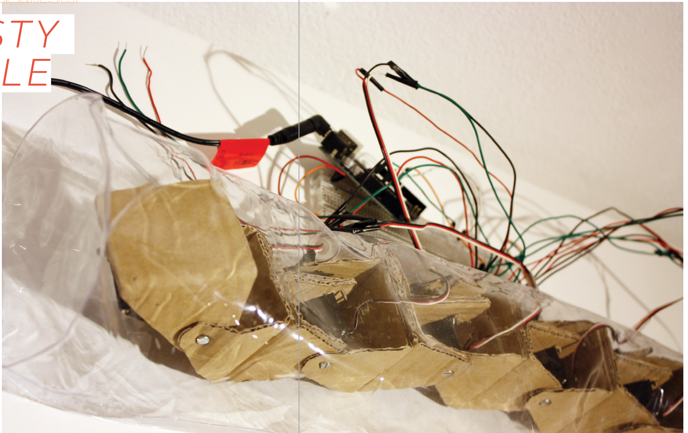
Fragment, 2010, Kirsty Boyle, modular robot (electronics, cardboard) variable dimensions. (Photographic documentation by Eser Aygün.)
